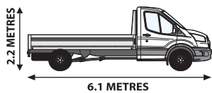
Ford Transit Tipper - P/LOAD: 1200 Kgs LOAD AREA: L 3.2 xW 2.1 Metres Towing Capacity 2800kgs / GTW 5500 Kgs
