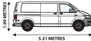
VW Transporter LWB - P/LOAD: 1000 Kgs LOAD AREA: L 2.8 x H 1.3 xW 1.5 Metres
