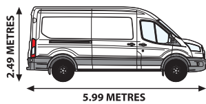
Ford Transit LWB - P/LOAD: 1600 Kgs LOAD AREA: L 3.4 xH 1.5 x W 1.5 Metres
