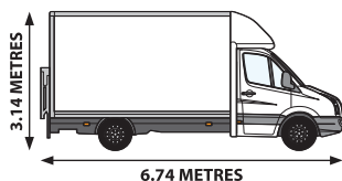
Luton T/L - P/LOAD: 1200 Kgs LOAD AREA: L 3.6 x H 2.1 xW 2.0 Metres
