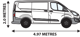
Ford Transit Custom - P/LOAD: 1000 Kgs LOAD AREA: L 2.4 x H 1.3 xW 1.4 Metres
