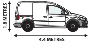
VW Caddy - P/LOAD: 650 Kgs LOAD AREA: L 1.7 x H 1.1 xW 1.4 Metres
