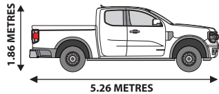
Ford Ranger - P/LOAD: 1200 Kgs LOAD AREA: L 1.5 xW 1.4 Metres Towing Capacity 3500kgs / GTW 5500 Kgs
